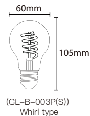
(GL-B-003P(S)) Whirl type
