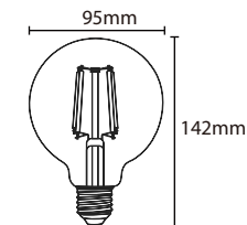
(GL-B-004P) Straight type
